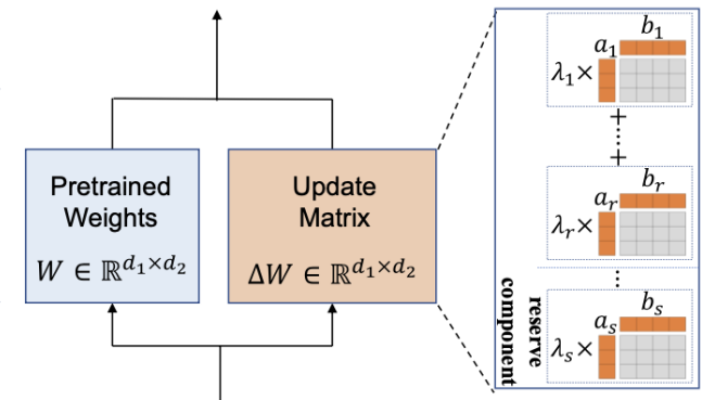
(c) IncreLoRA
