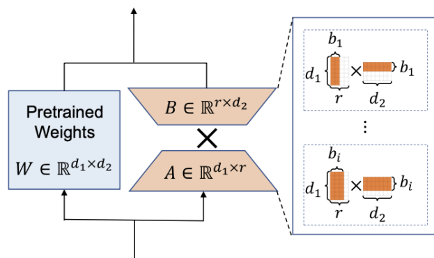
(a) DyLoRA
